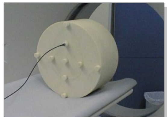
CTWater® CTDI phantom for assesement of dose in CT
